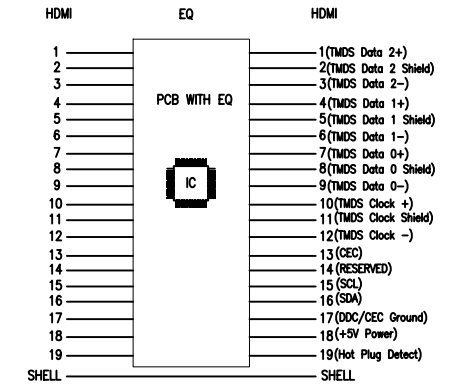
PIN ASSIGNMENT:
