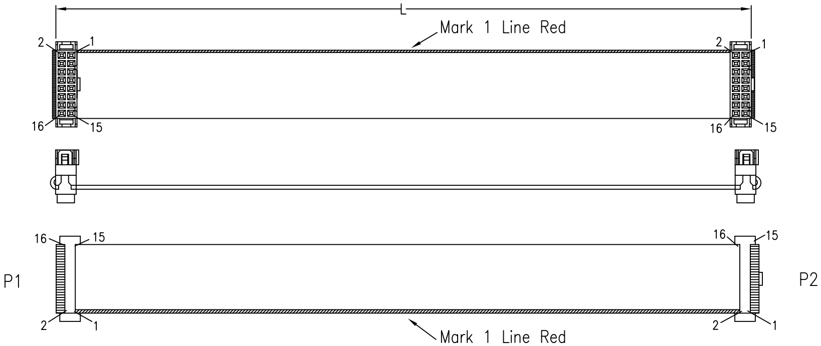
16P IDC CHART: WITH SR
