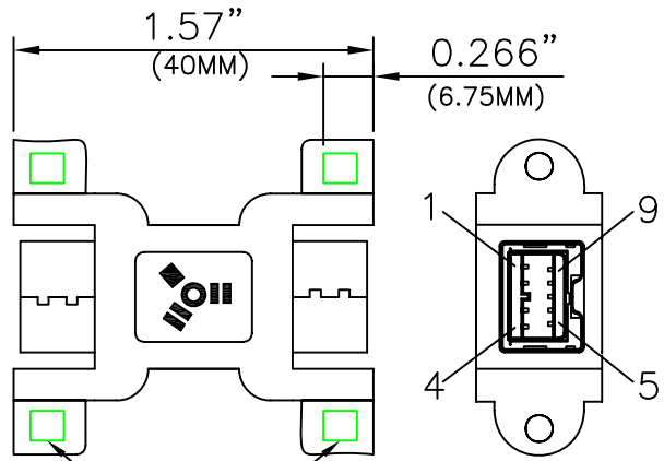
P2 1394 9P/F
