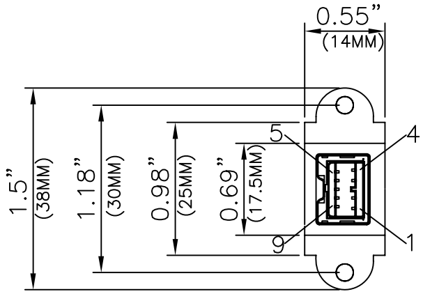
P1 1394 9P/F
