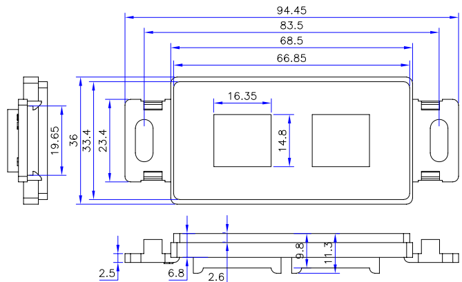
DECORA 2 PORT(07X-102-WH-J)
