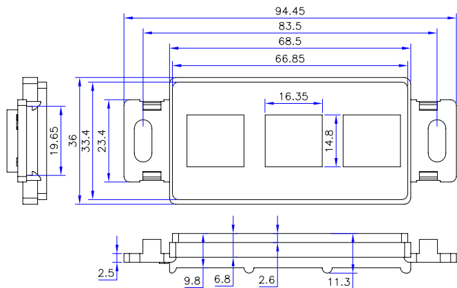
DECORA 3 PORT(07X-103-WH-J)
