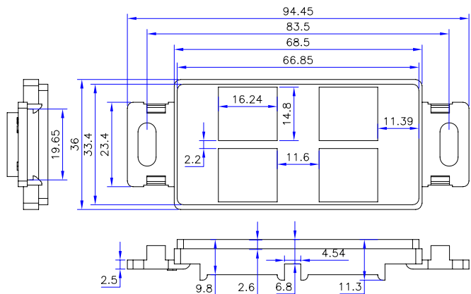
DECORA 4 PORT(07X-I04-WH-J)
