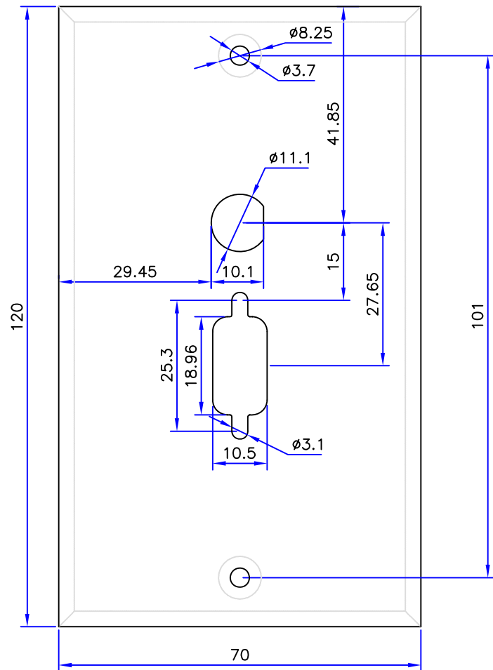
Punch size drawing
