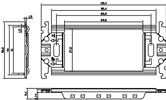
METAL FRAME
