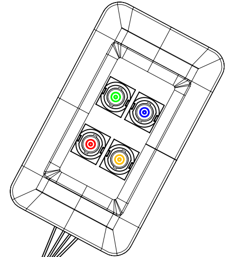
ASSEMBLY DRAWING
