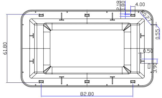
JAPANESE FACE PLATE(FRONT HOOD)
