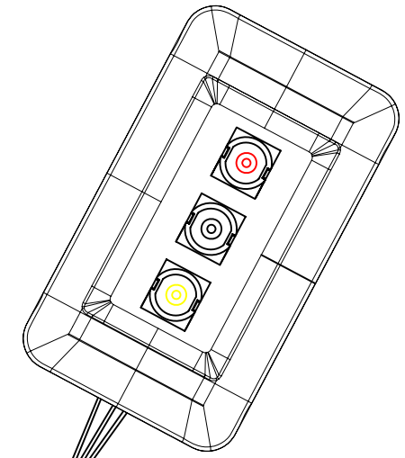
ASSEMBLY DRAWING
