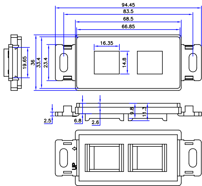
DECORA 2 PORT(07X-102-WH-J)
