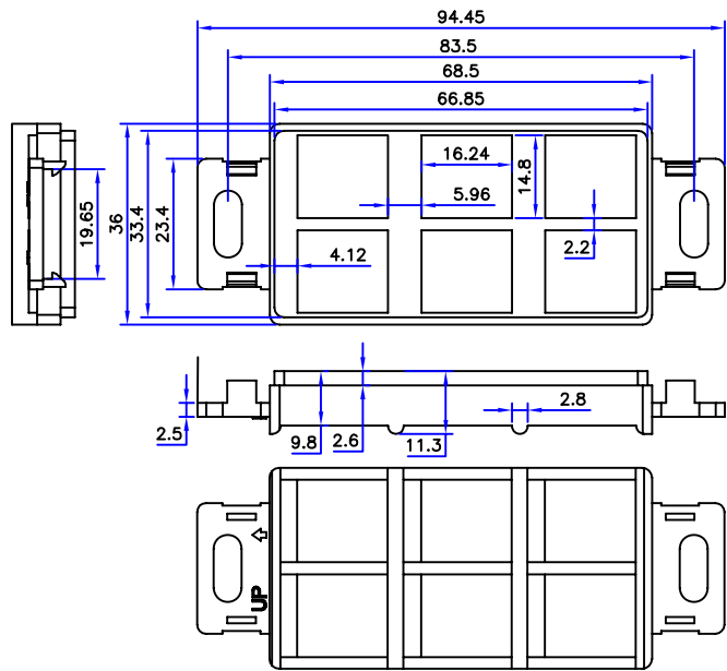
DECORA 6 PORT(07X-104-WH-J)
