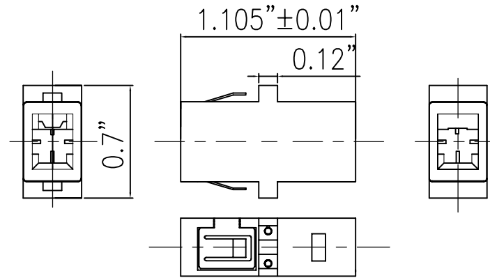
MTRJ F/F ADAPTER(UNIT:INCH)
