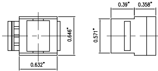
MODULE DRAWING(UNIT:INCH)
