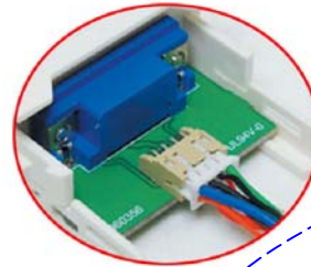
Pin Connection View
