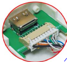
Pin Connection View
