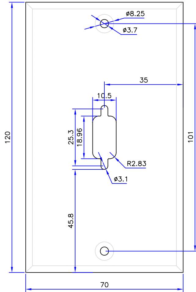
Punch size drawing
