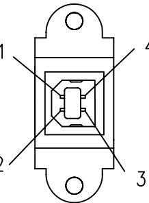
P2 USB B/F
