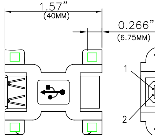
P2 USB B/F
