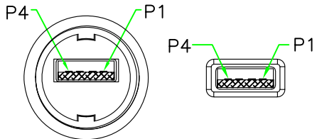
PIN ASSIGNMENT FRONT VIEW (前視圖)
