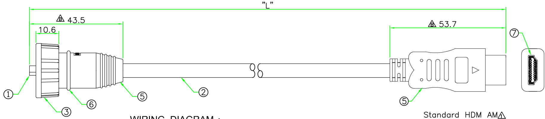
WIRING DIAGRAM \Delta
